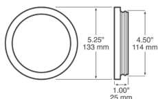
PM-1217G-R-426 flush mount
