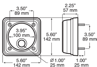
PM-1217G-R-417 surface mount
